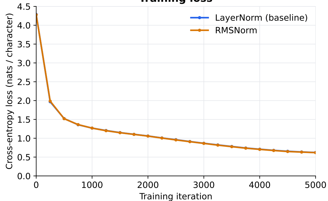
Training loss
